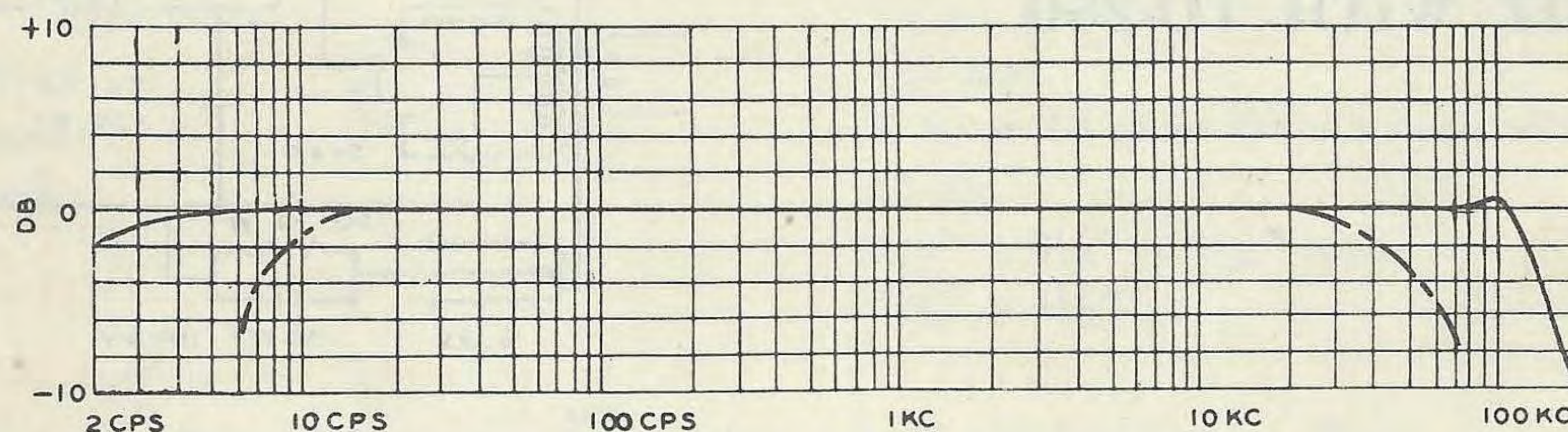
Frequency Response and Power Curves (frequency ————— power - - - - -)
