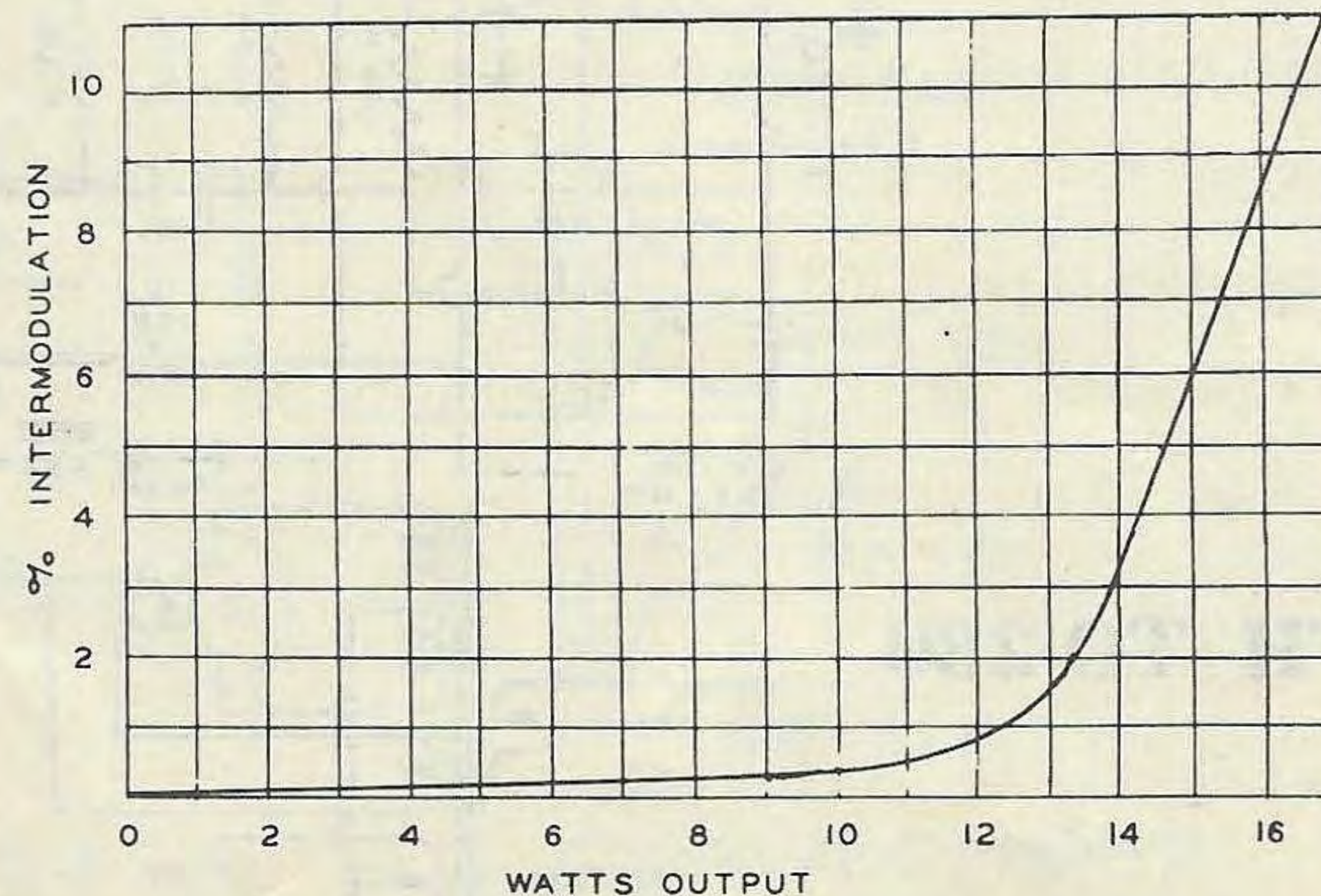
Intermodulation Distortion Versus Power (40 cps and 2,000 cps mixed 4:1)
