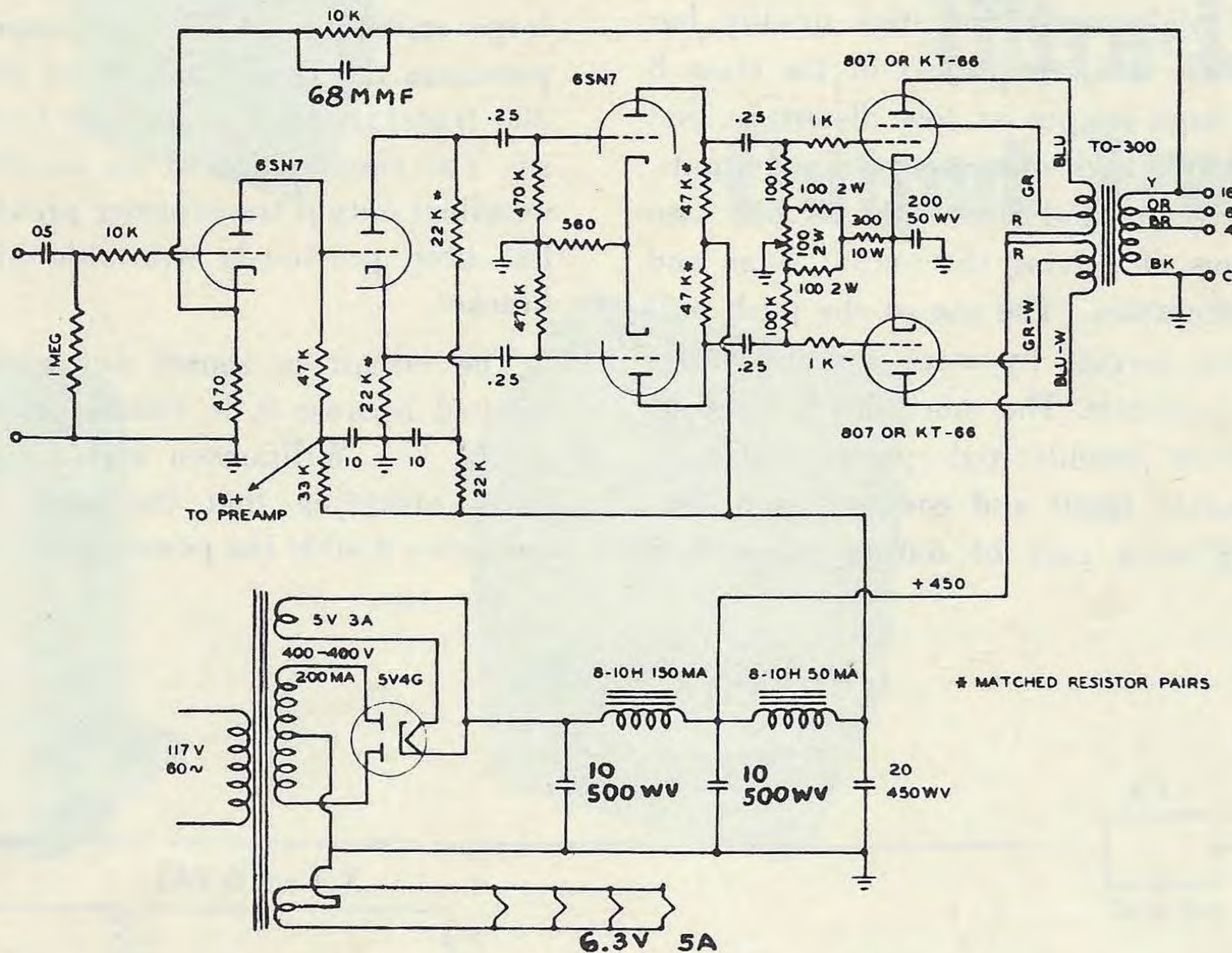
Circuit
