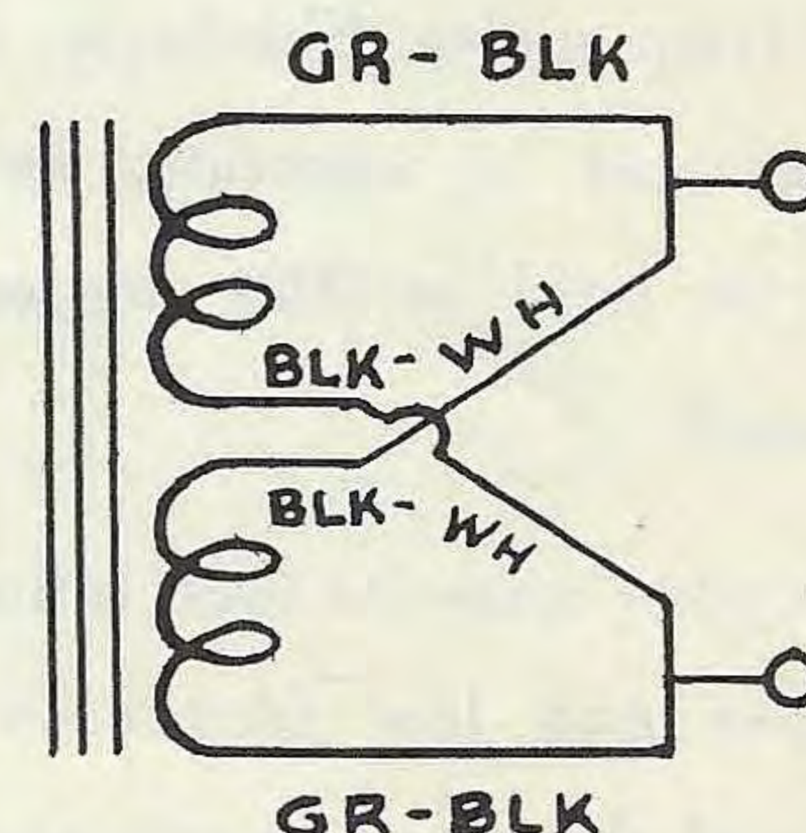
CONNECTIONS FOR 125 OHMS
