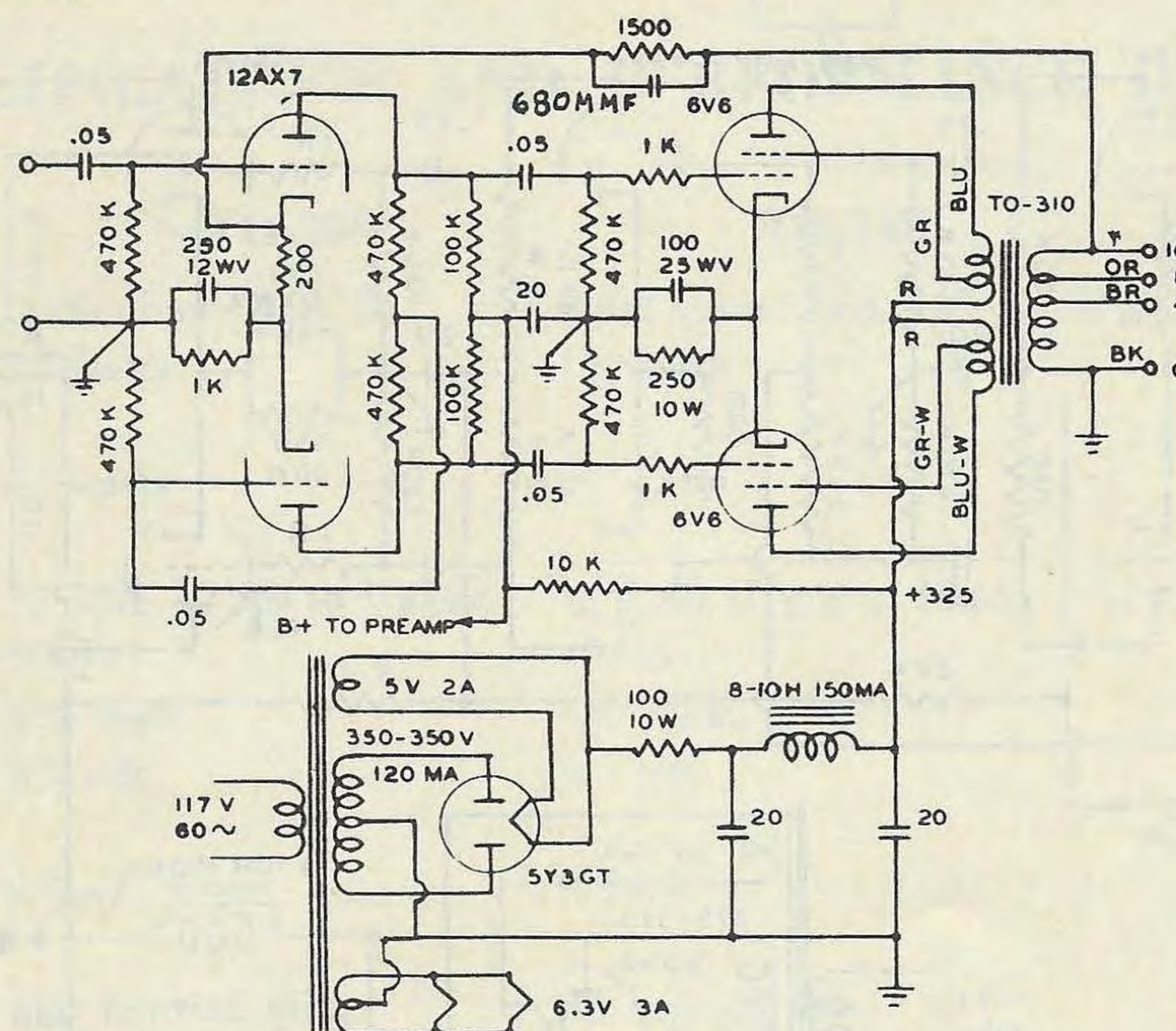
Circuit
